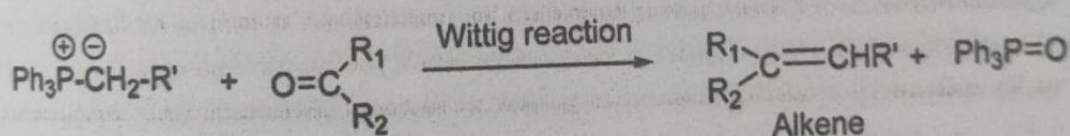
SCHEME 1 Wittig reaction
