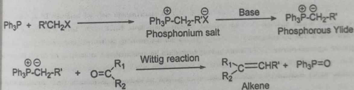
SCHEME 1 Wittig reaction
